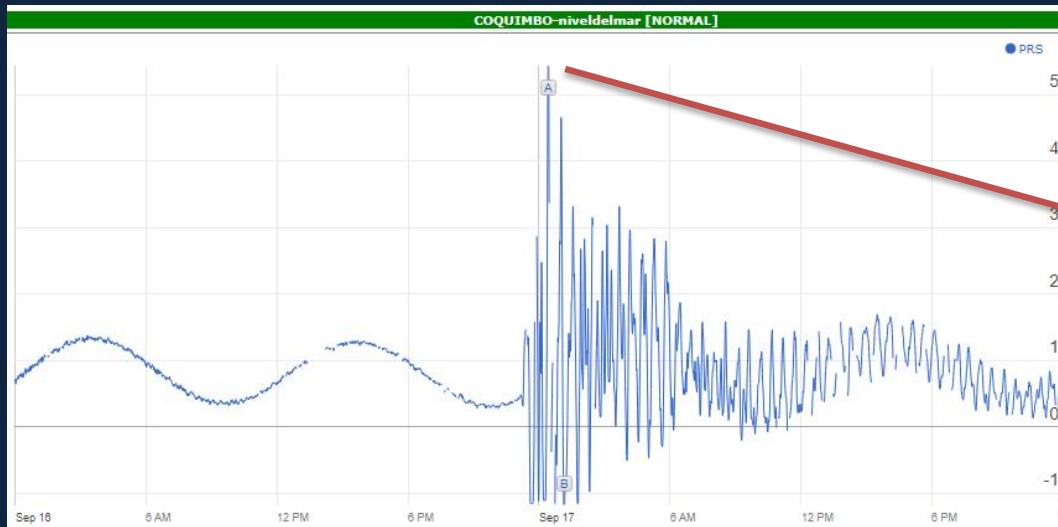
Data using GOES telemetry: 4.6m tsunami
